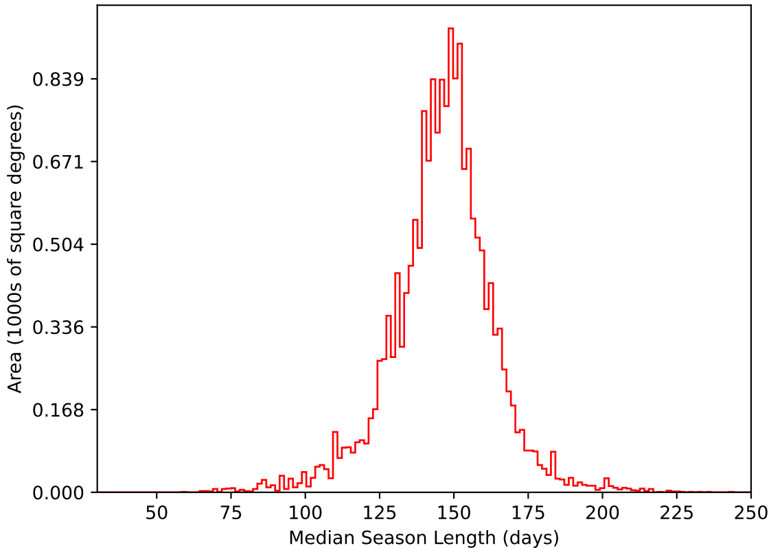
ddf_acor_sf15_lsf30_lsr10_v3.4_10yrs WFD i band: Median Season Length
