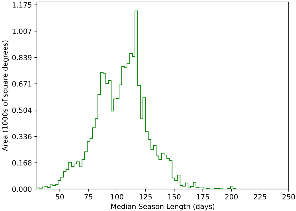
ddf_acor_sf15_ls30_lsr10_v3.4_10yrs WFD g band: Median Season Length
