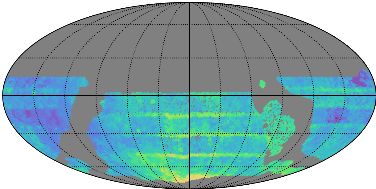
ddf_acor_sf15_lsf30_lsr10_v3.4_10yrs WFD all bands: Median Season Length
