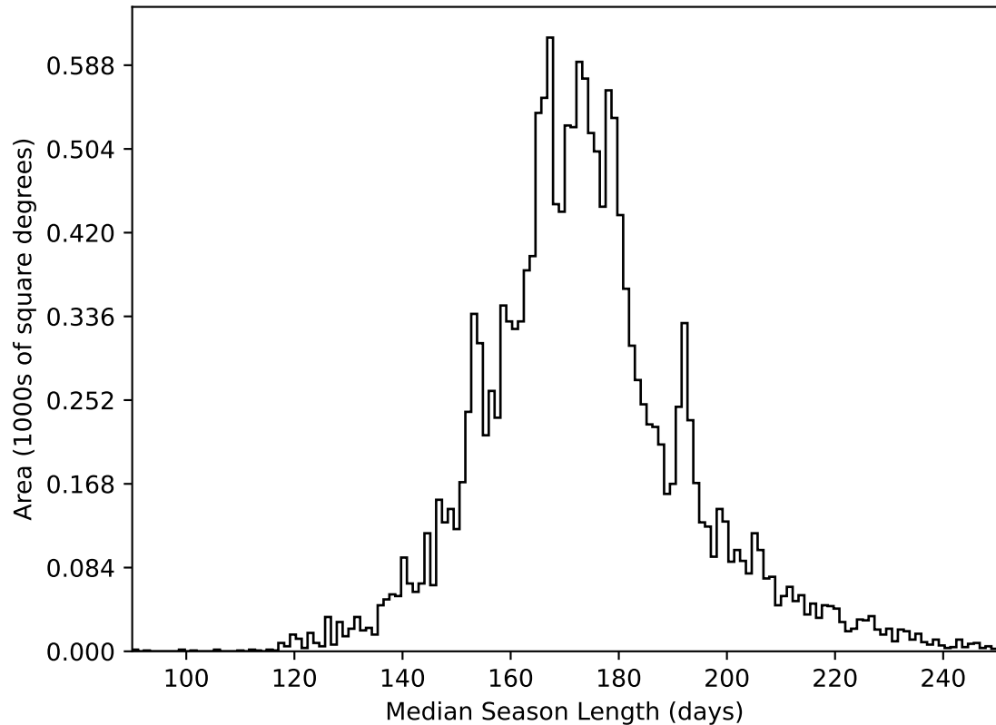
ddf_acor_sf15_lsf30_lsr10_v3.4_10yrs WFD all bands: Median Season Length
