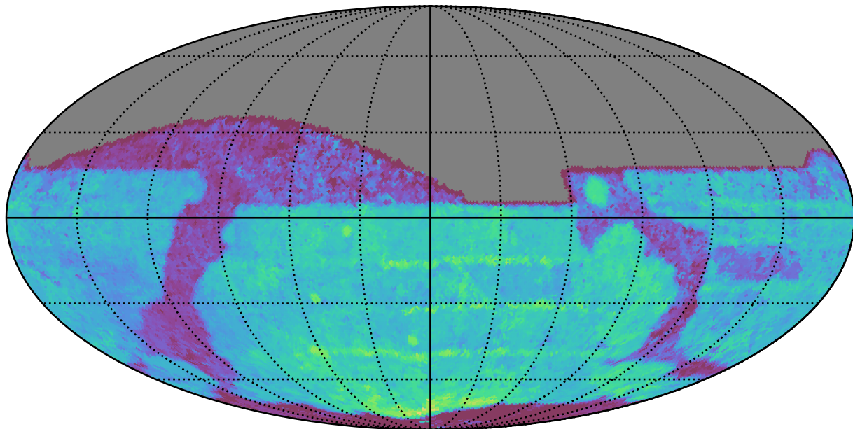
ddf_acor_sf15_lsf30_lsr10_v3.4_10yrs All sky z band: Median Season Length
