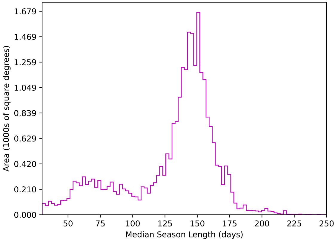
ddf_acor_sf15_lsf30_lsr10_v3.4_10yrs All sky z band: Median Season Length
