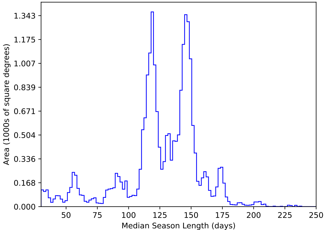
ddf_acor_sf15_lsf30_lsr10_v3.4_10yrs All sky y band: Median Season Length
