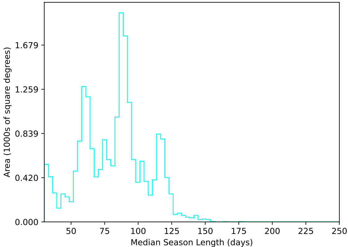
ddf_acor_sf15_lsf30_lsr10_v3.4_10yrs All sky u band: Median Season Length
