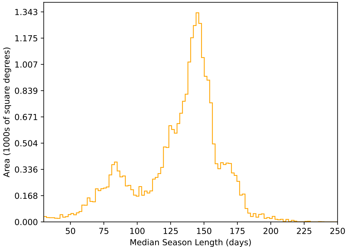
ddf_acor_sf15_lsf30_lsr10_v3.4_10yrs All sky r band: Median Season Length
