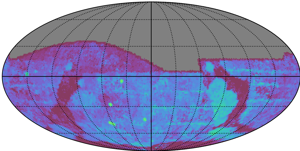
ddf_acor_sf15_lsf30_lsr10_v3.4_10yrs All sky g band: Median Season Length
