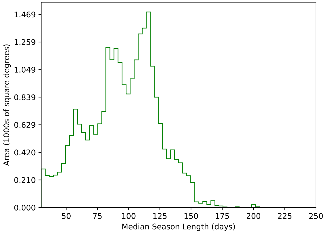
ddf_acor_sf15_lsf30_lsr10_v3.4_10yrs All sky g band: Median Season Length
