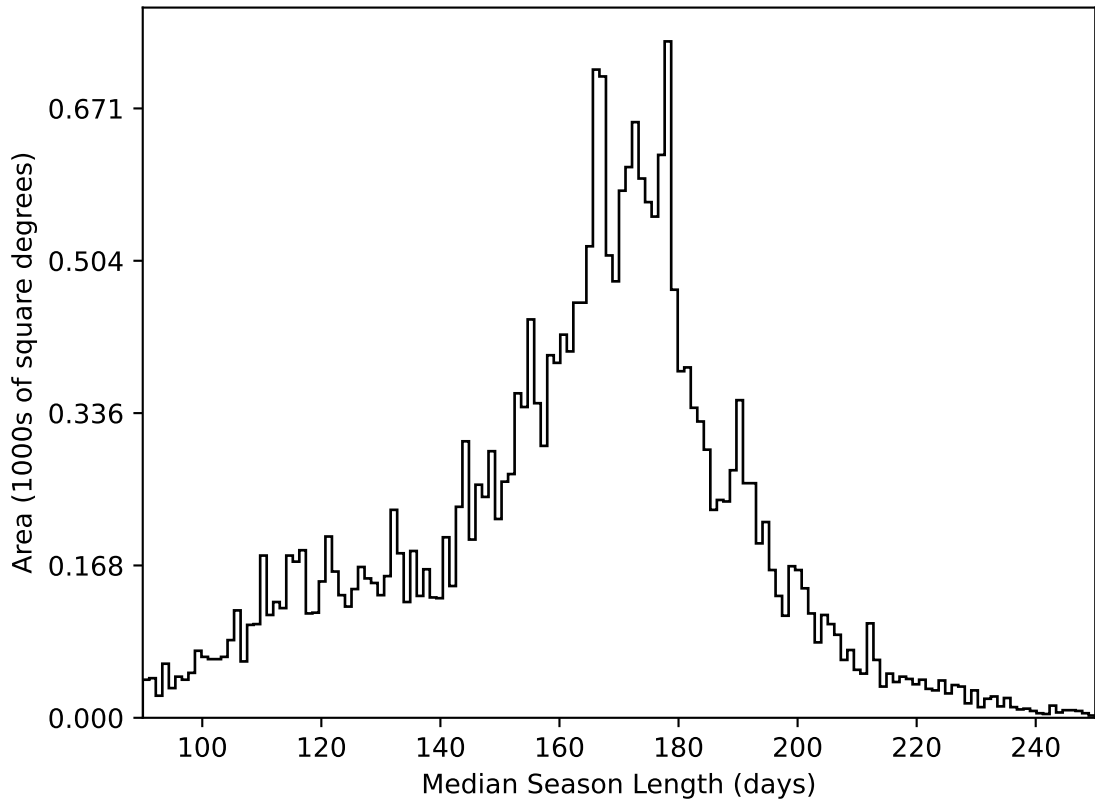
ddf_acor_sf15_lsf30_lsr10_v3.4_10yrs All sky all bands: Median Season Length
