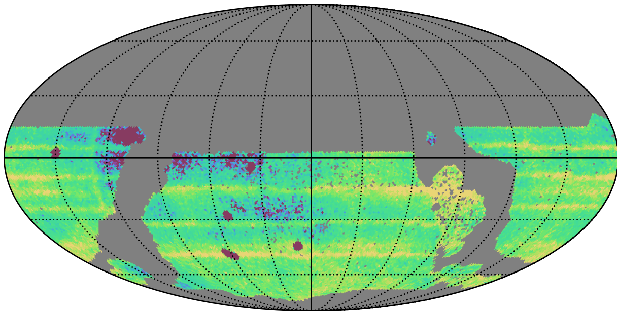
ddf_acor_sf15_lsf30_lsr10_v3.4_10yrs WFD: Median Intra-Night Gap
