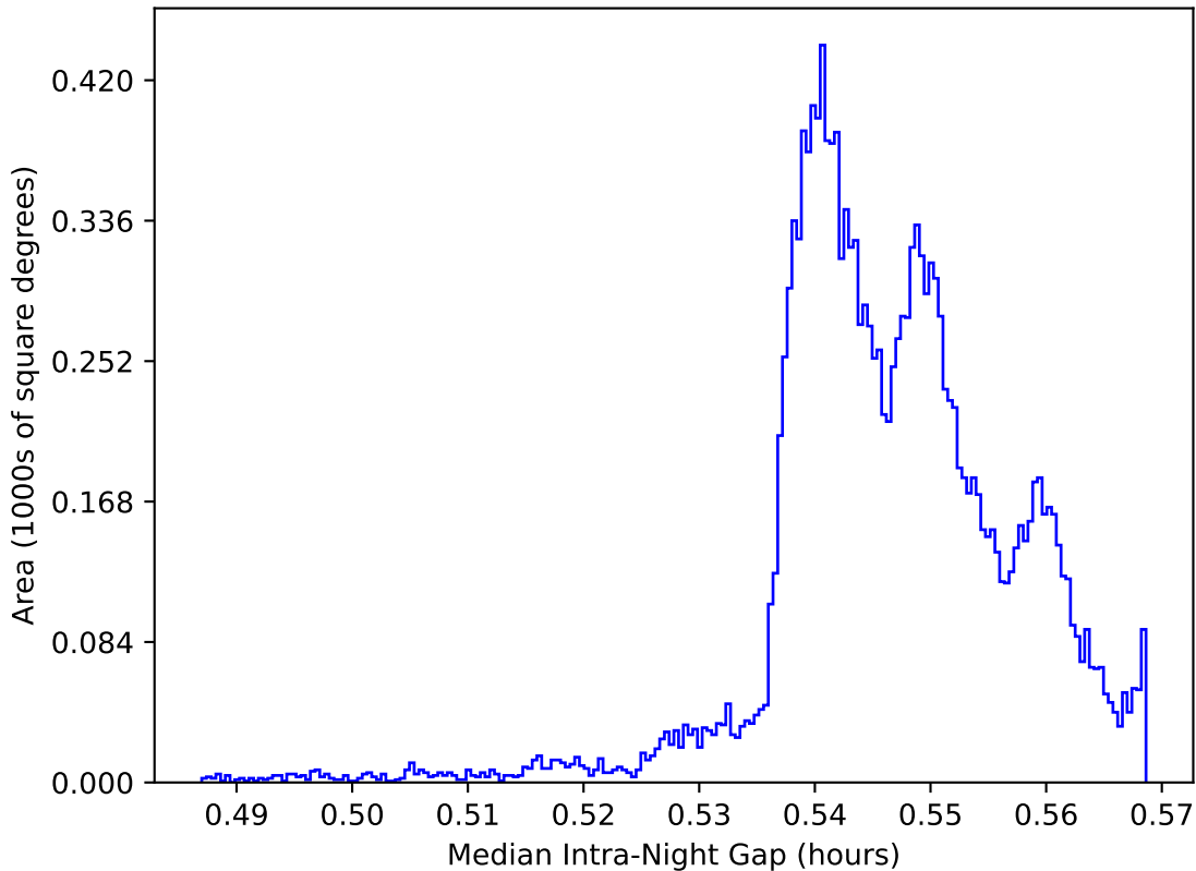
ddf_acor_sf15_lsf30_lsr10_v3.4_10yrs WFD: Median Intra-Night Gap
