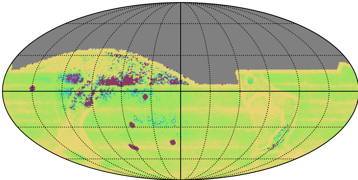
ddf_acor_sf15_lsf30_lsr10_v3.4_10yrs All sky: Median Intra-Night Gap
