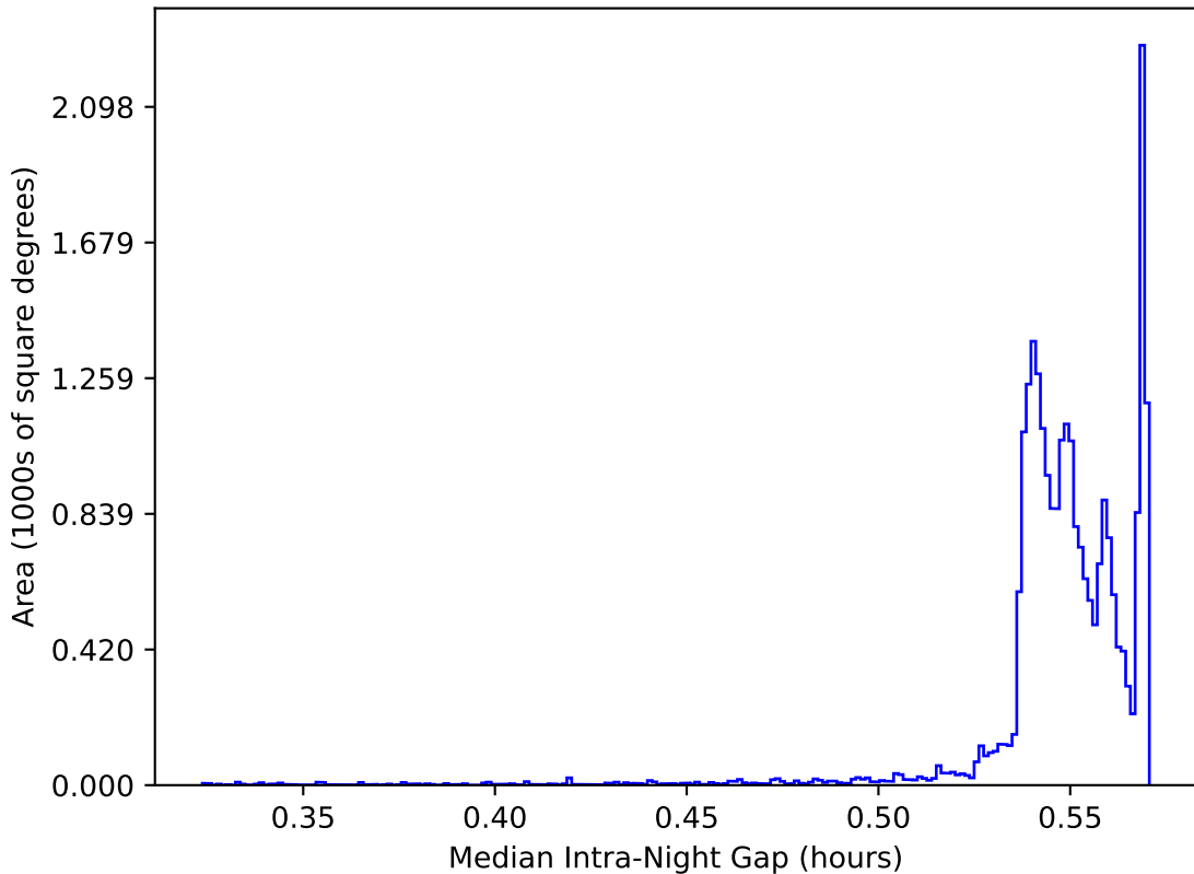
ddf_acor_sf15_lsf30_lsr10_v3.4_10yrs All sky: Median Intra-Night Gap
