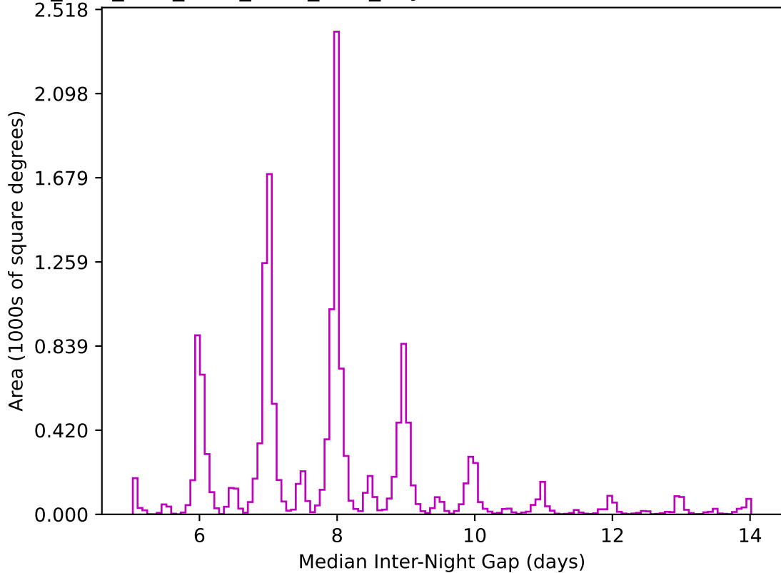
ddf_acor_sf15_lsf30_lsr10_v3.4_10yrs WFD z band: Median Inter-Night Gap
