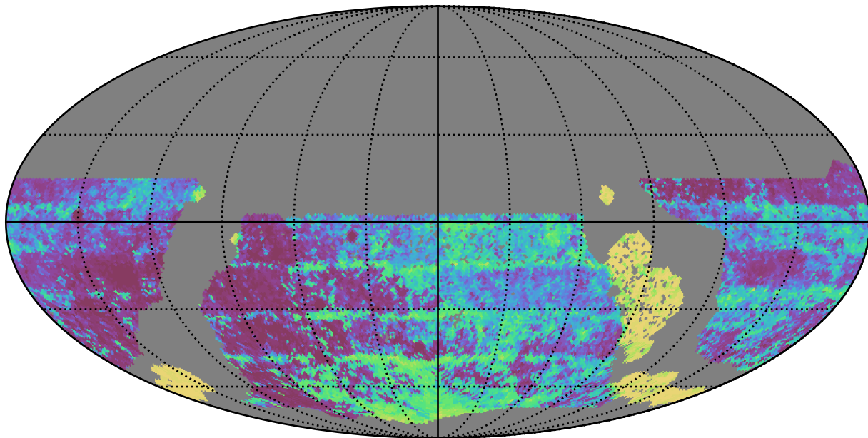
ddf_acor_sf15_lsf30_lsr10_v3.4_10yrs WFD y band: Median Inter-Night Gap
