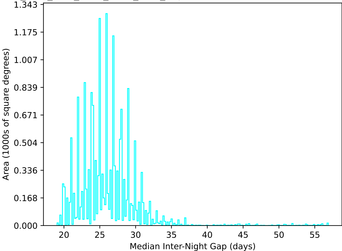
ddf_acor_sf15_lsf30_lsr10_v3.4_10yrs WFD u band: Median Inter-Night Gap
