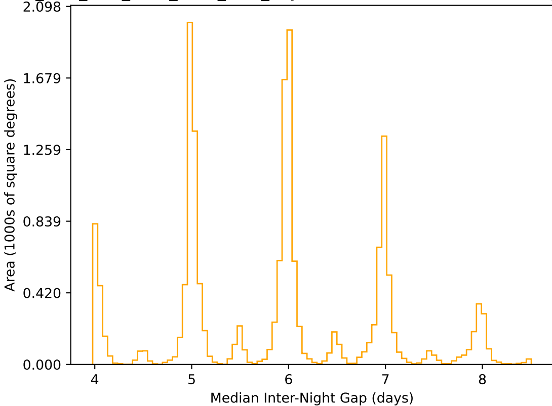
ddf_acor_sf15_ls30_lsr10_v3.4_10yrs WFD r band: Median Inter-Night Gap
