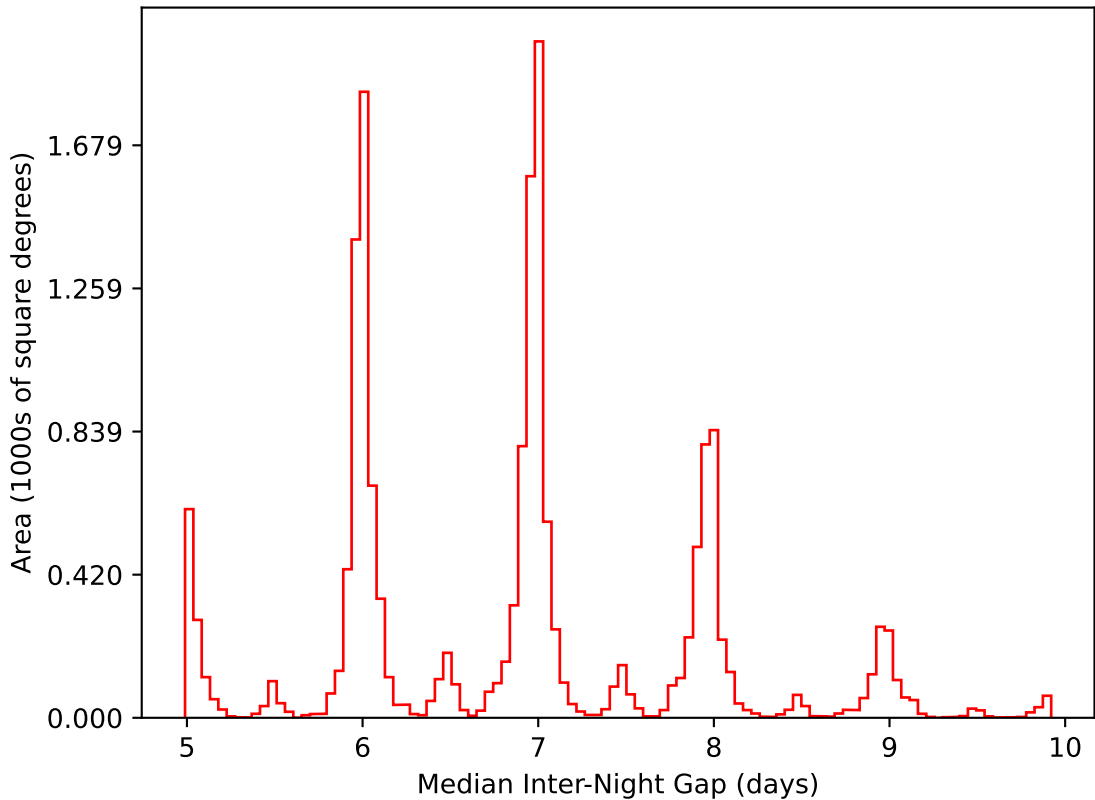
ddf_acor_sf15_ls30_lsr10_v3.4_10yrs WFD i band: Median Inter-Night Gap
