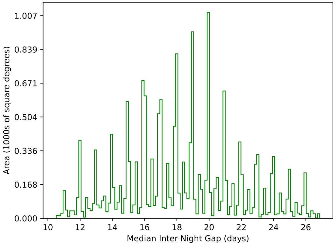
ddf_acor_sf15_lsf30_lsr10_v3.4_10yrs WFD g band: Median Inter-Night Gap
