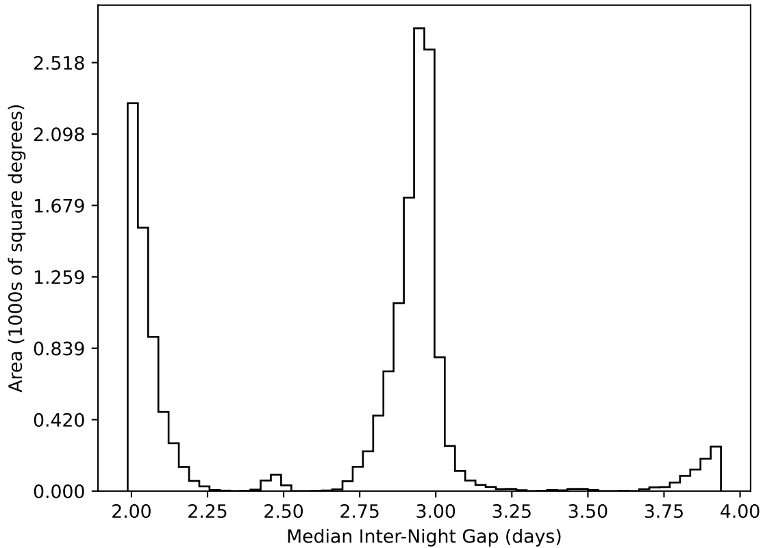
ddf_acor_sf15_lsf30_lsr10_v3.4_10yrs WFD all bands: Median Inter-Night Gap
