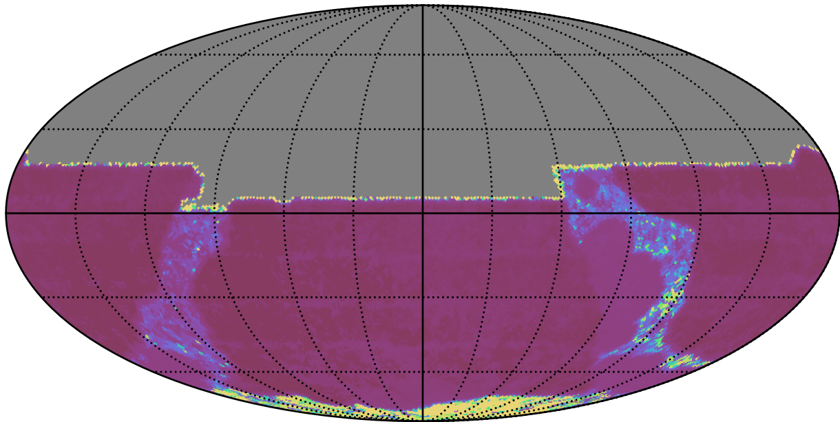
ddf_acor_sf15_lsf30_lsr10_v3.4_10yrs All sky y band: Median Inter-Night Gap
