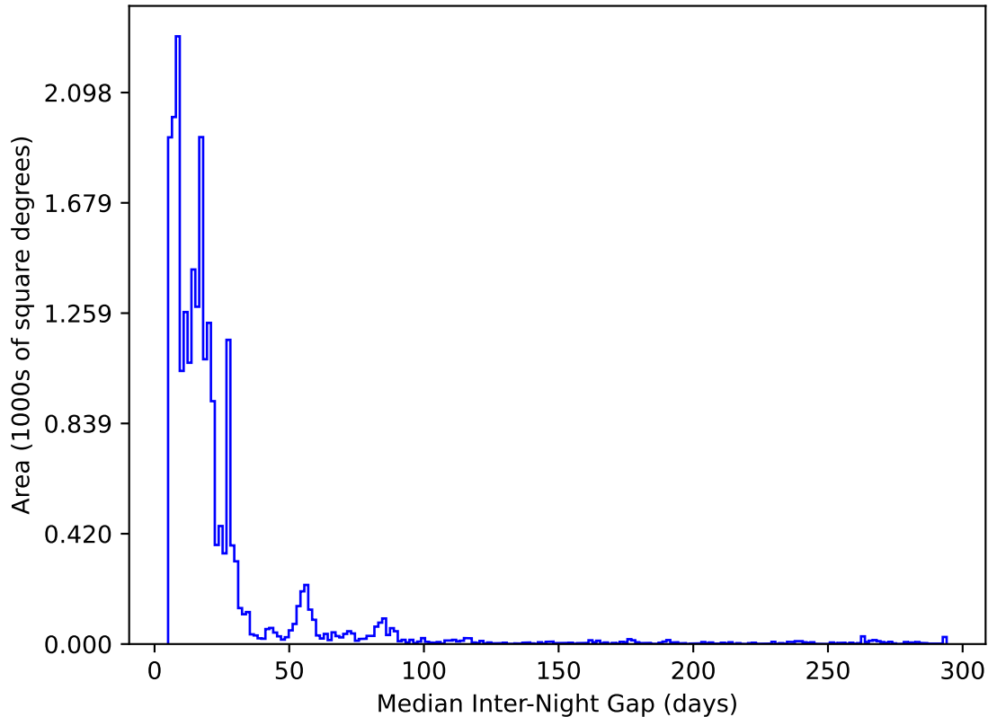
ddf_acor_sf15_lsf30_lsr10_v3.4_10yrs All sky y band: Median Inter-Night Gap
