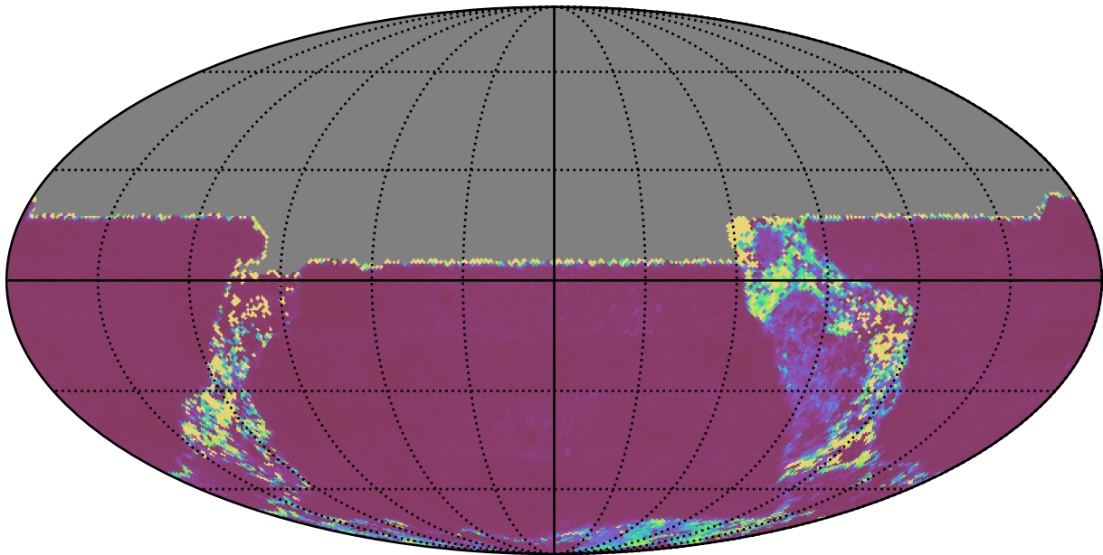
ddf_acor_sf15_lsf30_lsr10_v3.4_10yrs All sky u band: Median Inter-Night Gap
