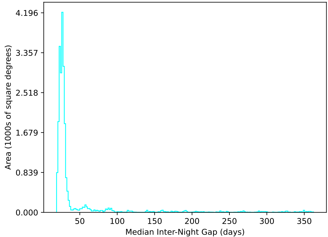
ddf_acor_sf15_lsf30_lsr10_v3.4_10yrs All sky u band: Median Inter-Night Gap
