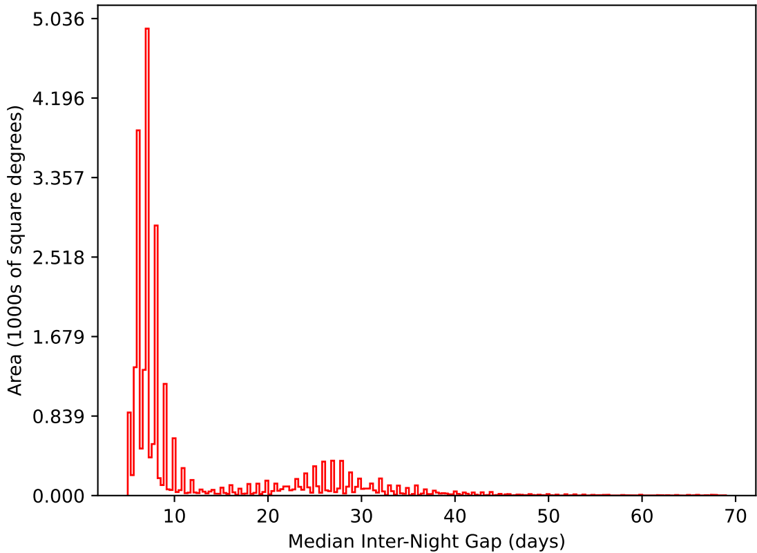
ddf_acor_sf15_lsf30_lsr10_v3.4_10yrs All sky i band: Median Inter-Night Gap
