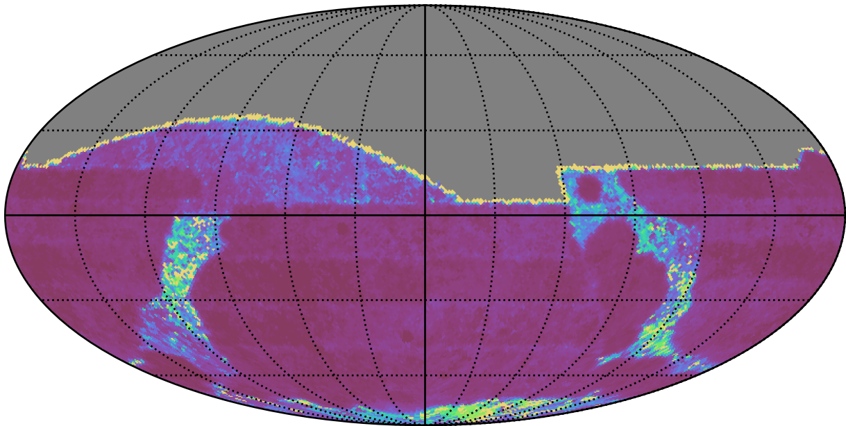
ddf_acor_sf15_lsf30_lsr10_v3.4_10yrs All sky g band: Median Inter-Night Gap
