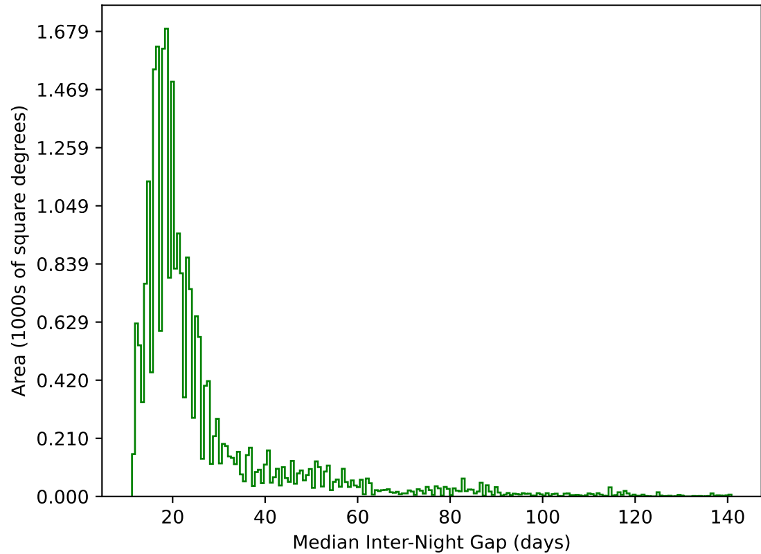
ddf_acor_sf15_lsf30_lsr10_v3.4_10yrs All sky g band: Median Inter-Night Gap
