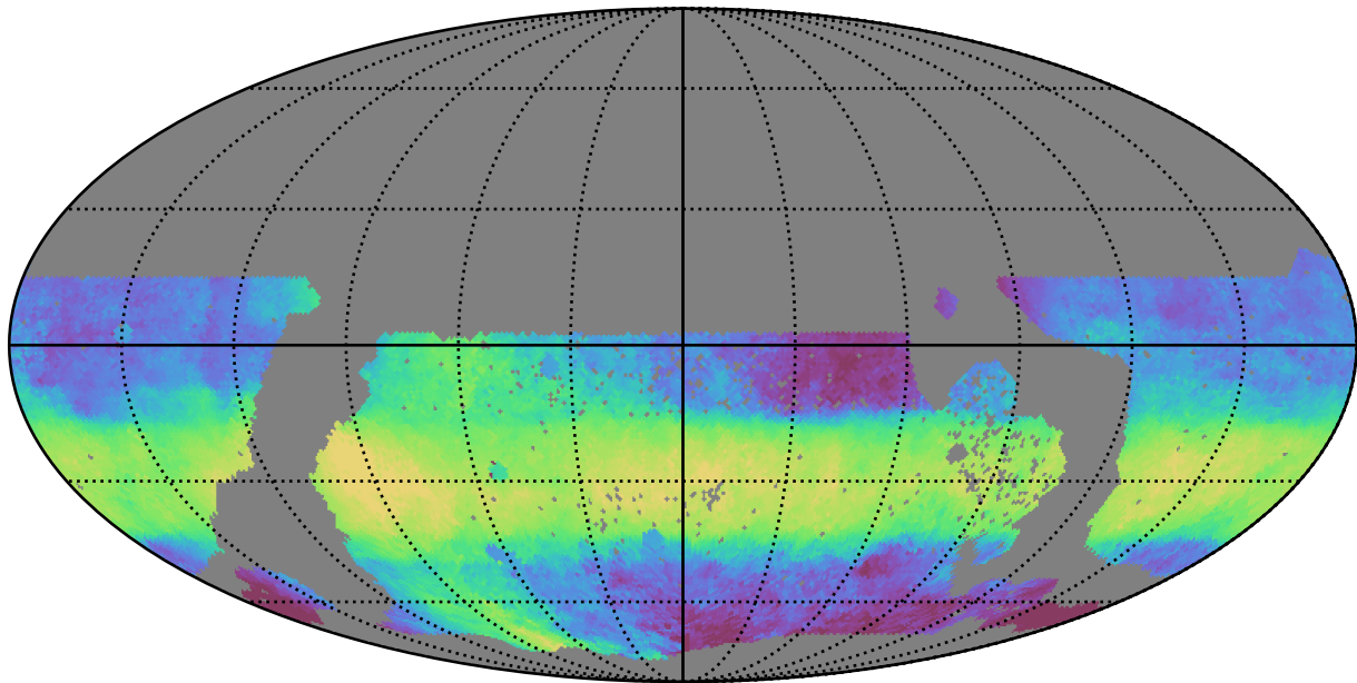
ddf_acor_sf15_lsf30_lsr10_v3.4_10yrs WFD z band: Median HA
