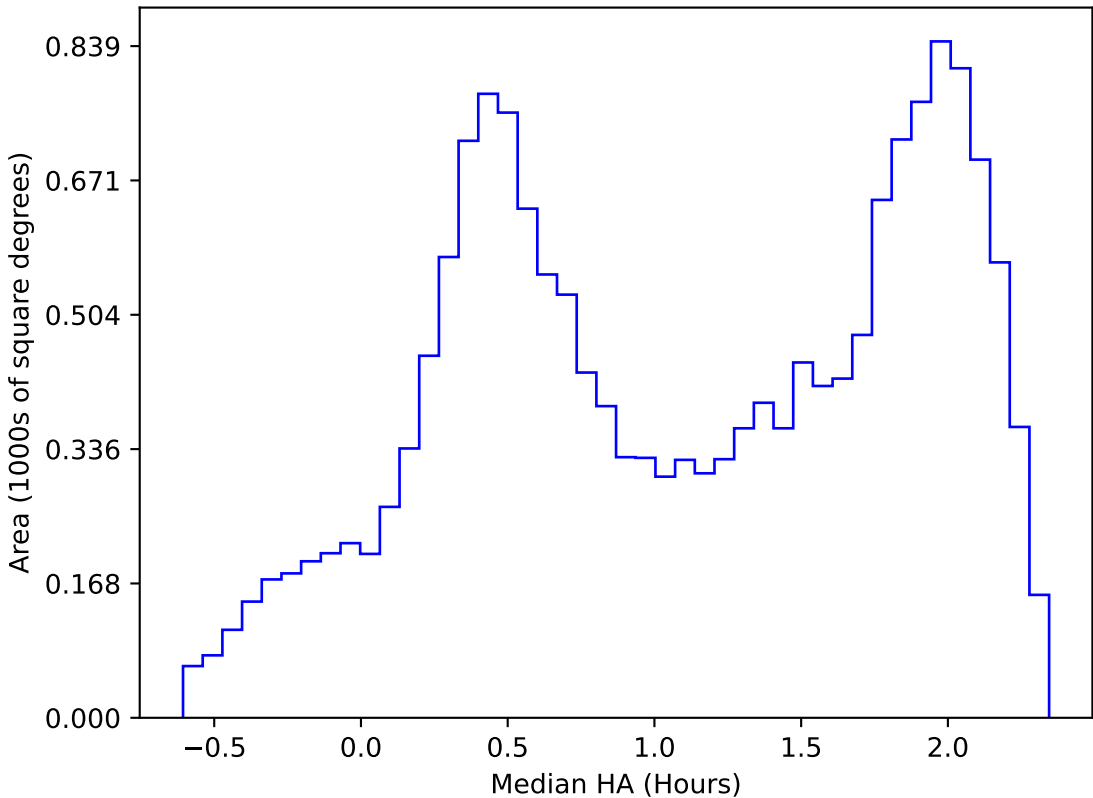
ddf_acor_sf15_lsf30_lsr10_v3.4_10yrs WFD z band: Median HA
