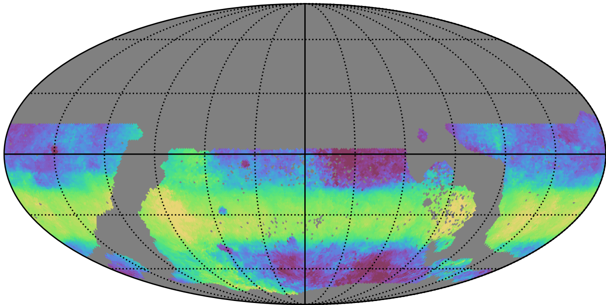
ddf_acor_sf15_lsf30_lsr10_v3.4_10yrs WFD y band: Median HA
