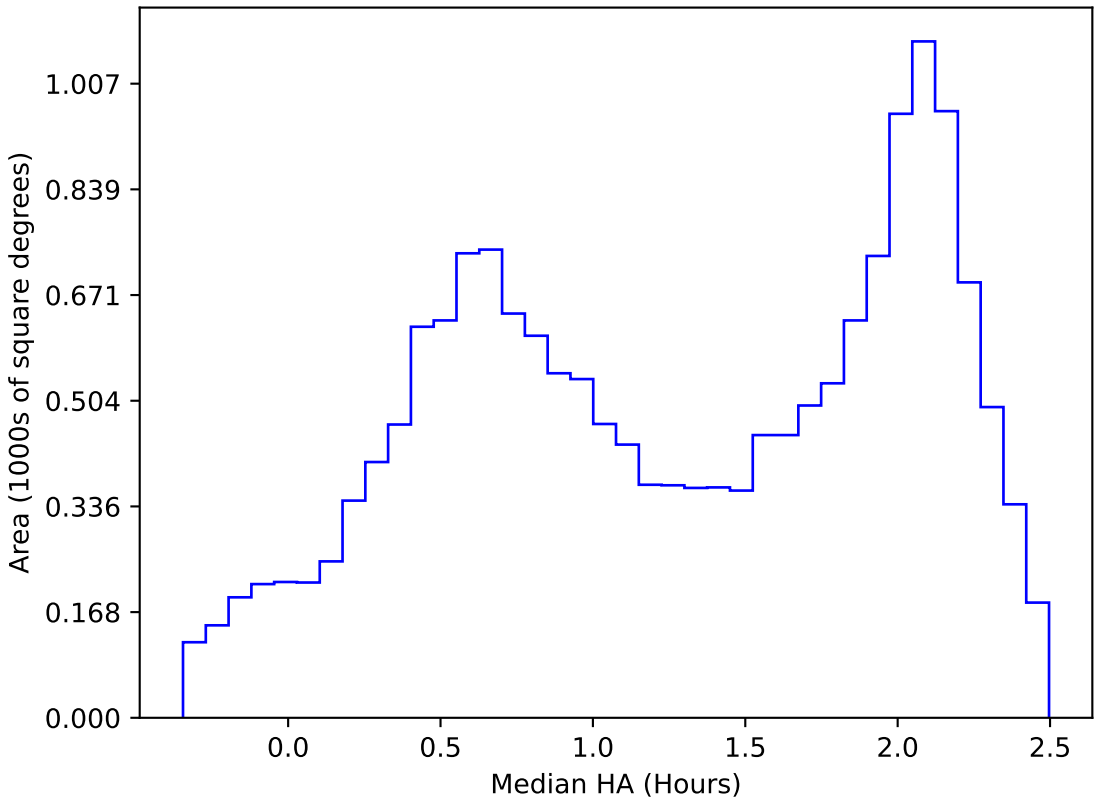
ddf_acor_sf15_lsf30_lsr10_v3.4_10yrs WFD y band: Median HA
