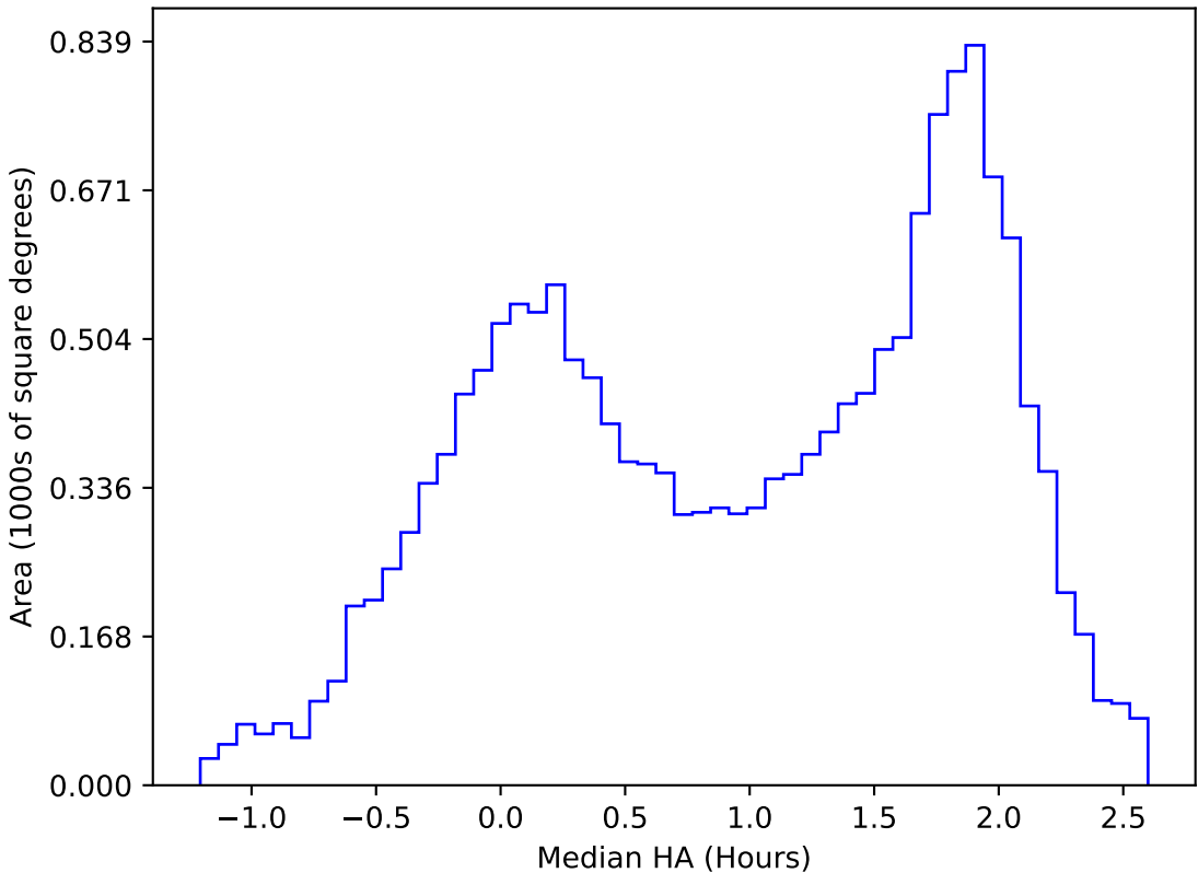
ddf_acor_sf15_lsf30_lsr10_v3.4_10yrs WFD u band: Median HA
