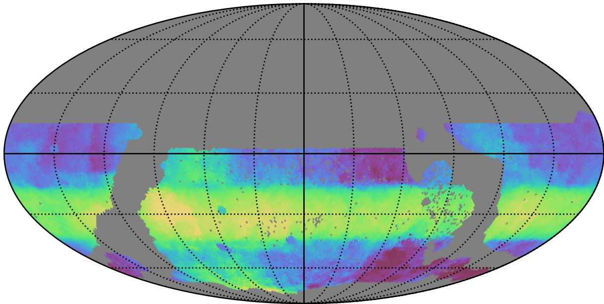
ddf_acor_sf15_lsf30_lsr10_v3.4_10yrs WFD r band: Median HA
