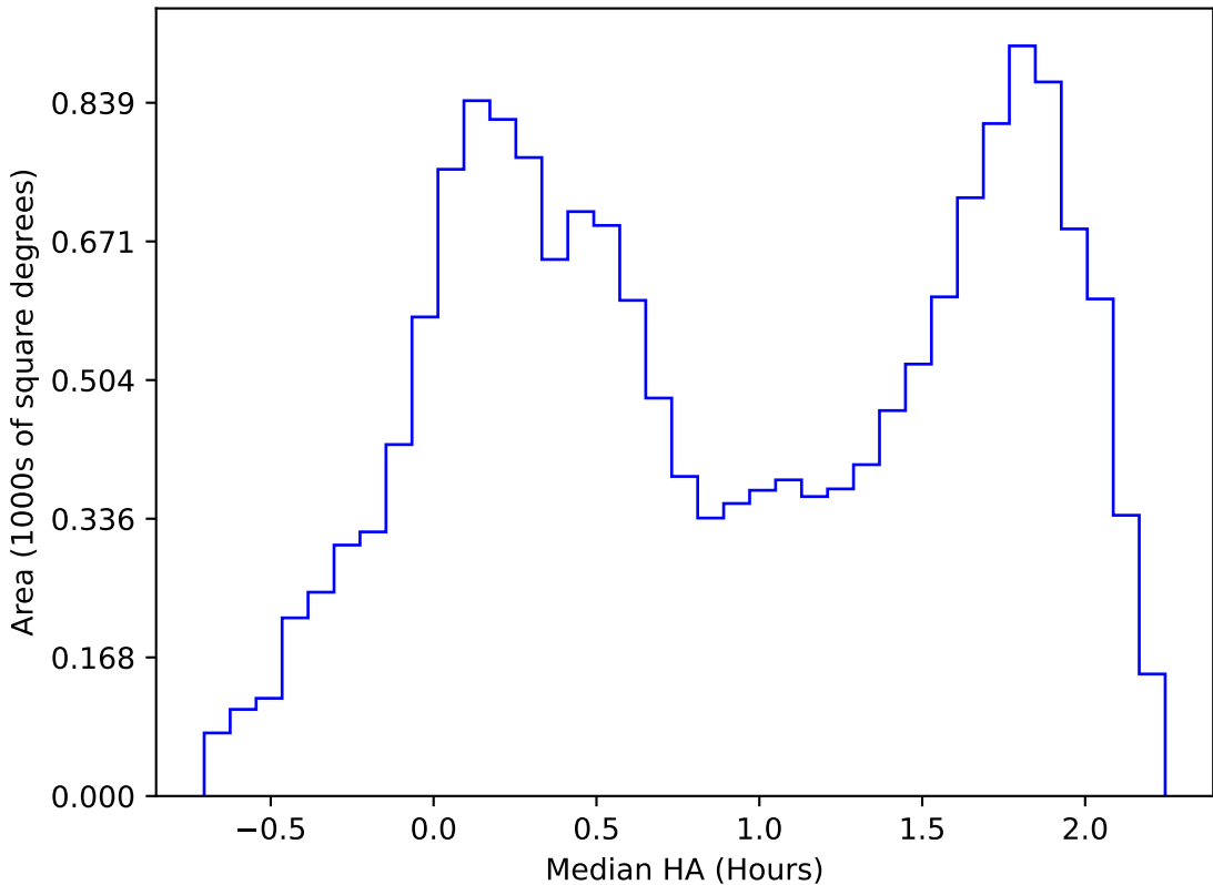
ddf_acor_sf15_lsf30_lsr10_v3.4_10yrs WFD r band: Median HA
