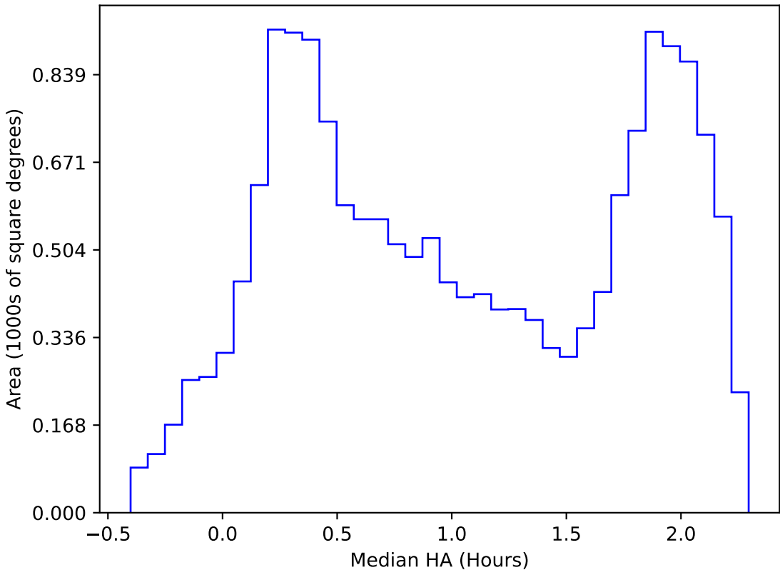
ddf_acor_sf15_lsf30_lsr10_v3.4_10yrs WFD i band: Median HA
