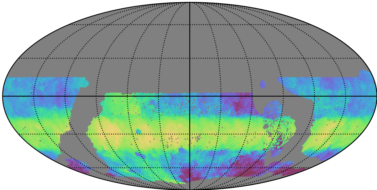
ddf_acor_sf15_lsf30_lsr10_v3.4_10yrs WFD g band: Median HA
