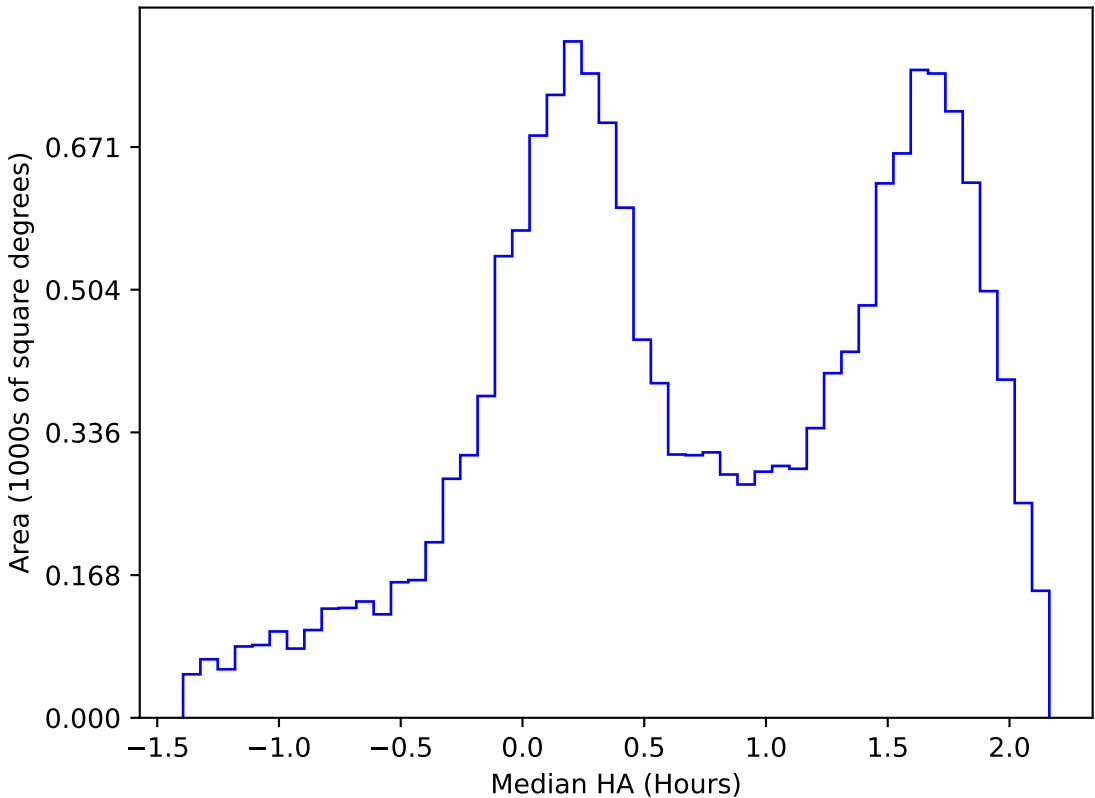
ddf_acor_sf15_lsf30_lsr10_v3.4_10yrs WFD g band: Median HA
