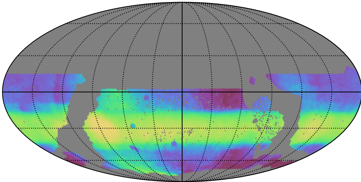
ddf_acor_sf15_lsf30_lsr10_v3.4_10yrs WFD all bands: Median HA
