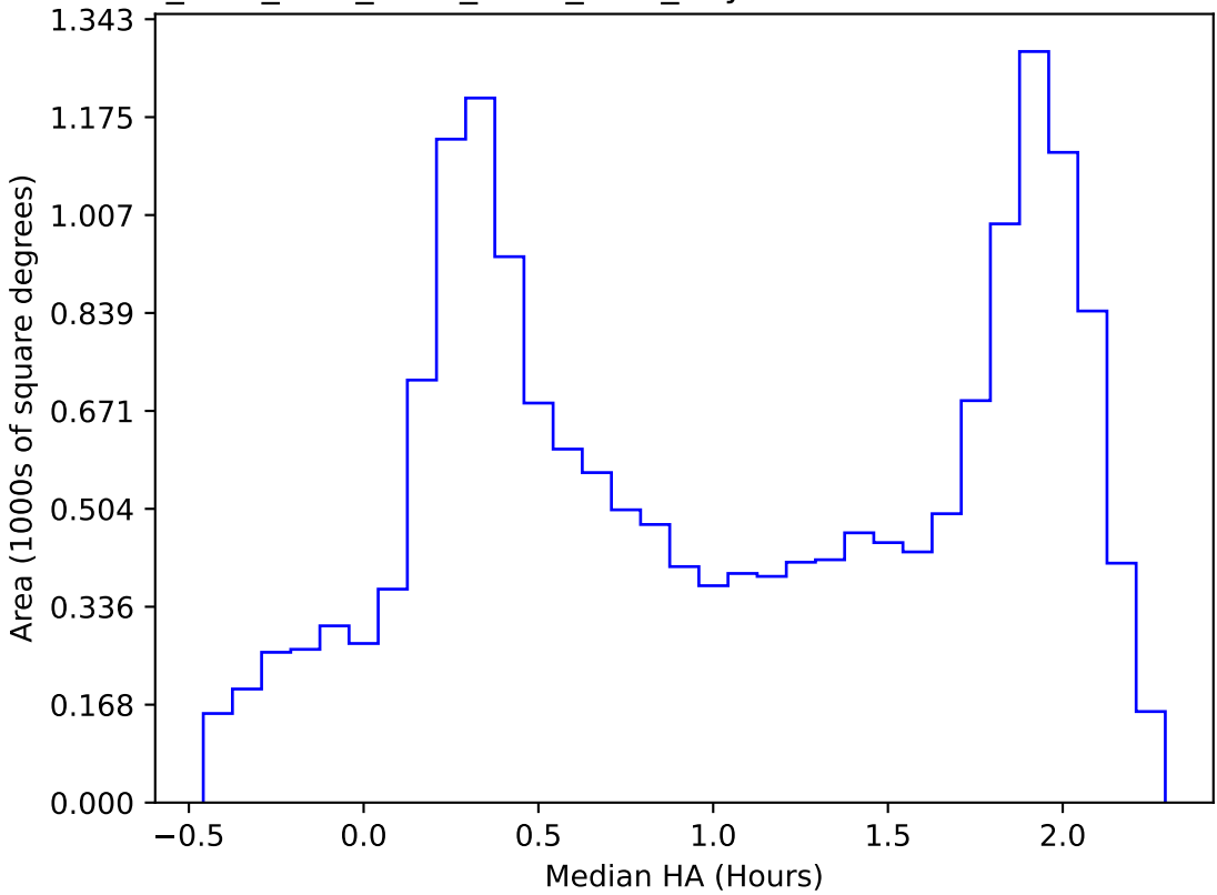
ddf_acor_sf15_lsf30_lsr10_v3.4_10yrs WFD all bands: Median HA
