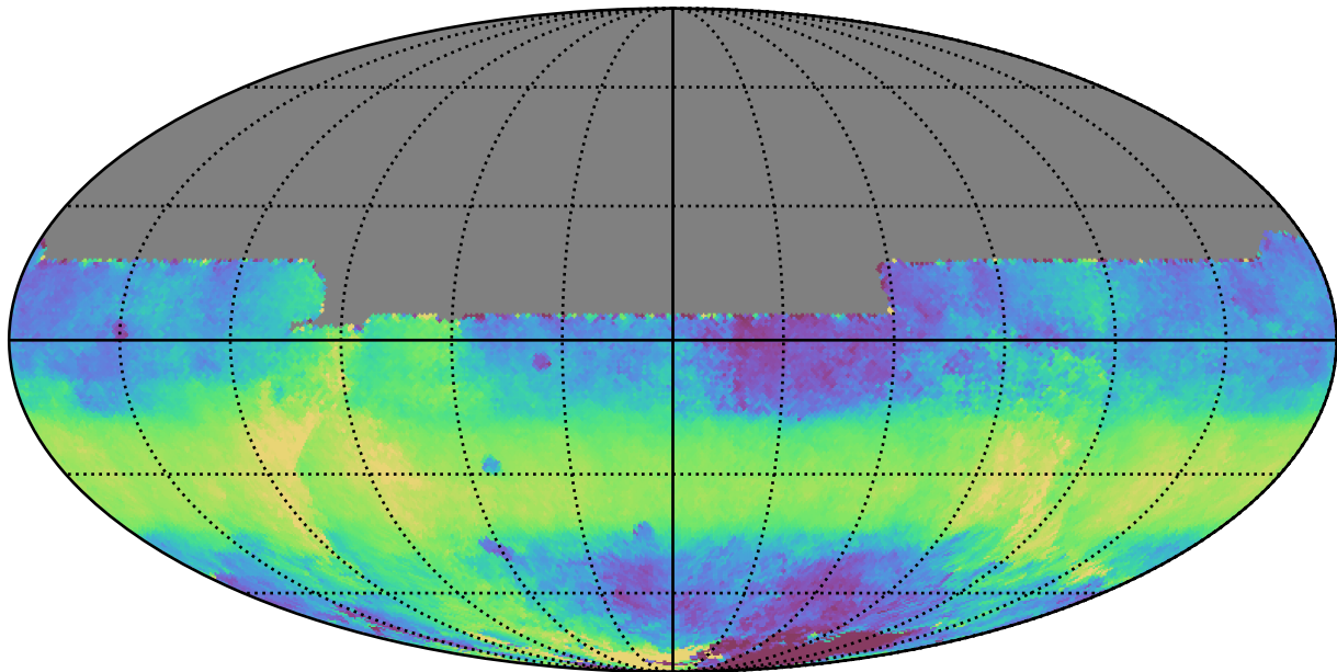
ddf_acor_sf15_lsf30_lsr10_v3.4_10yrs All sky y band: Median HA
