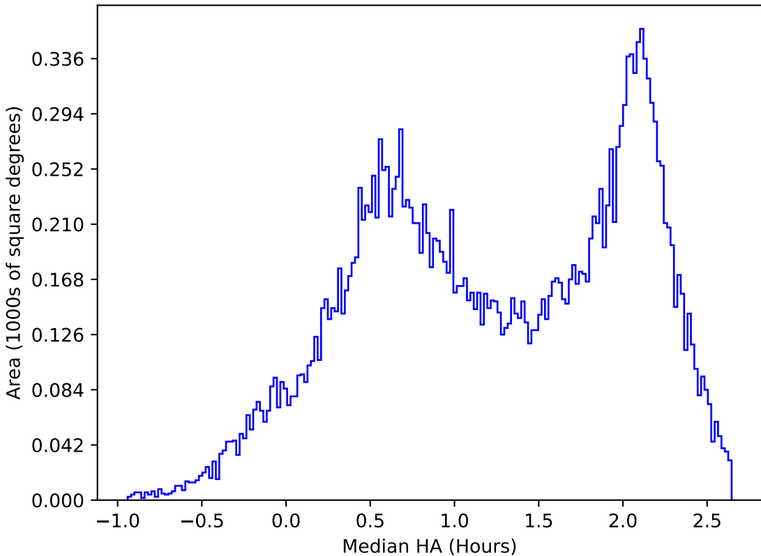
ddf_acor_sf15_ls30_lsr10_v3.4_10yrs All sky y band: Median HA
