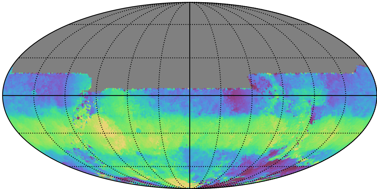
ddf_acor_sf15_lsf30_lsr10_v3.4_10yrs All sky u band: Median HA
