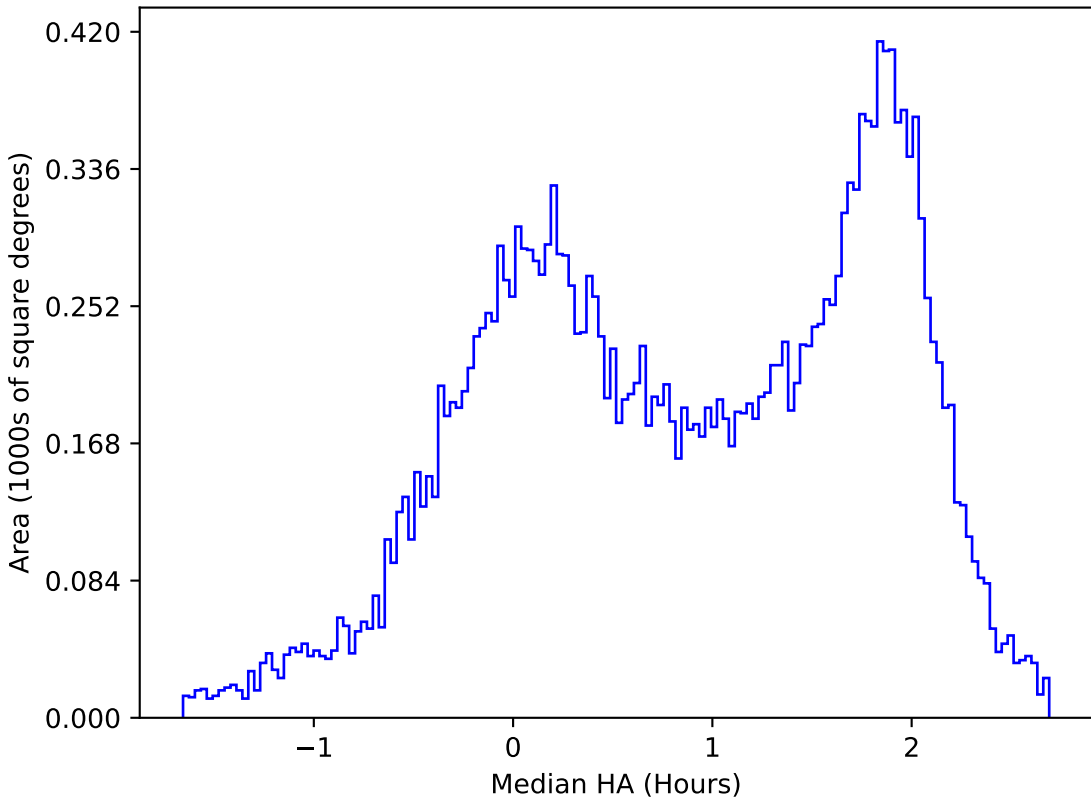
ddf_acor_sf15_ls30_lsr10_v3.4_10yrs All sky u band: Median HA
