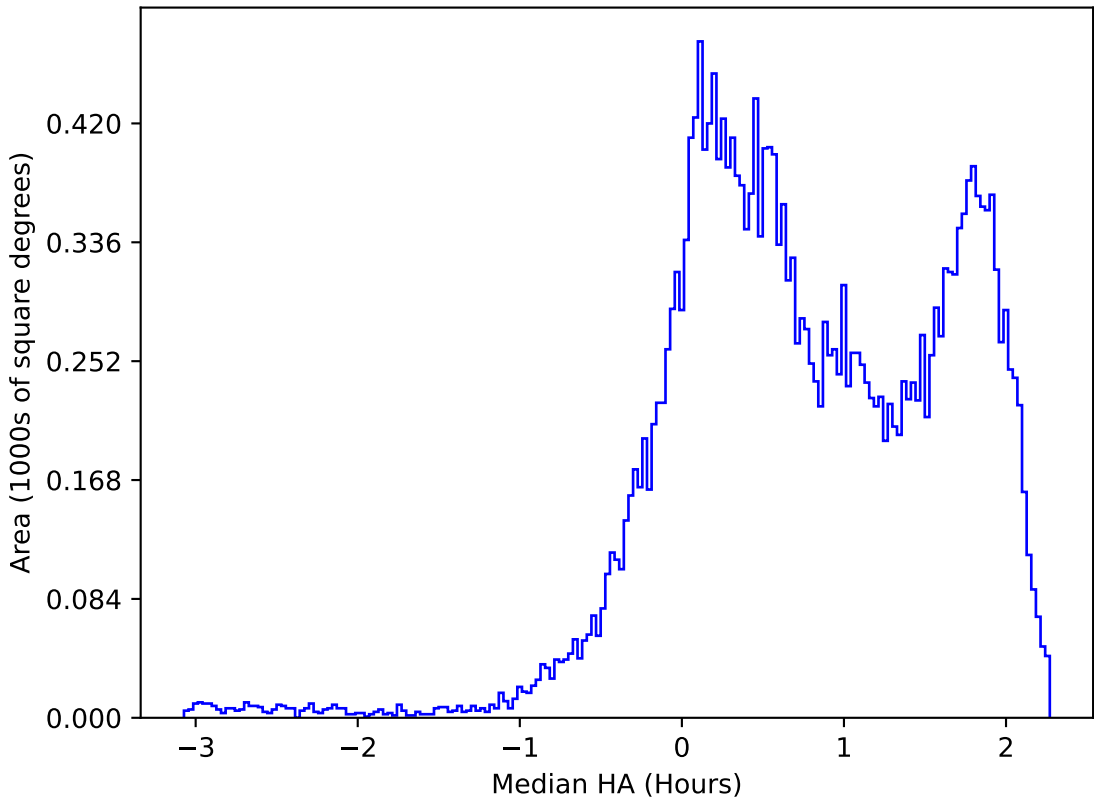
ddf_acor_sf15_lsf30_lsr10_v3.4_10yrs All sky r band: Median HA
