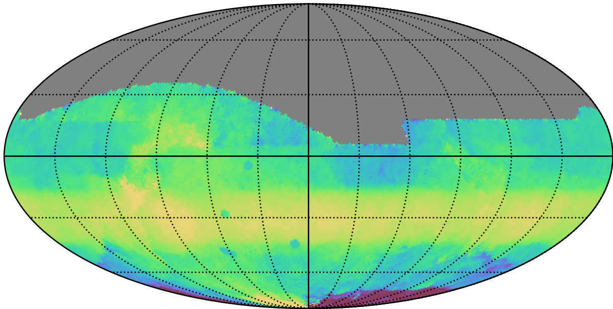
ddf_acor_sf15_lsf30_lsr10_v3.4_10yrs All sky i band: Median HA
