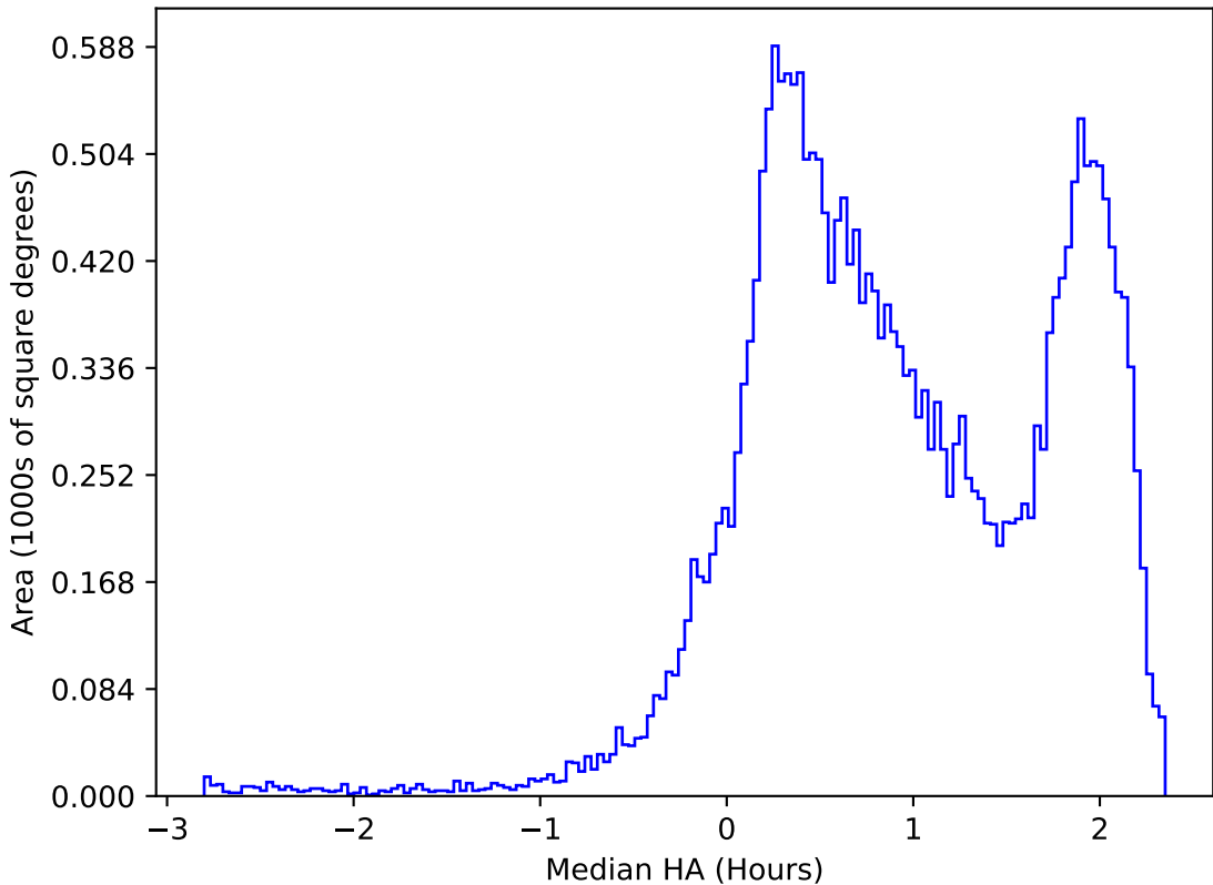
ddf_acor_sf15_lsf30_lsr10_v3.4_10yrs All sky i band: Median HA
