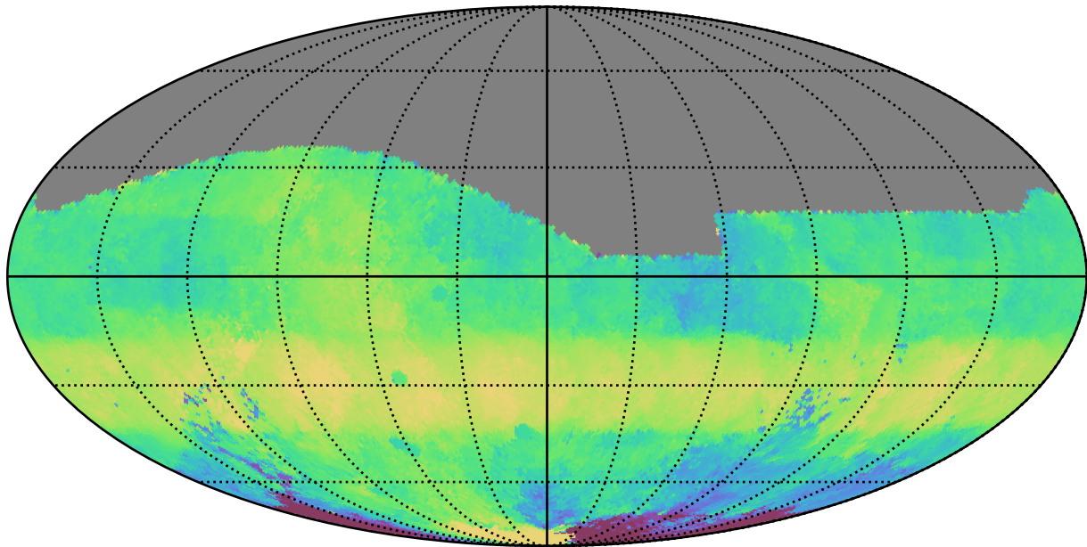
ddf_acor_sf15_lsf30_lsr10_v3.4_10yrs All sky g band: Median HA
